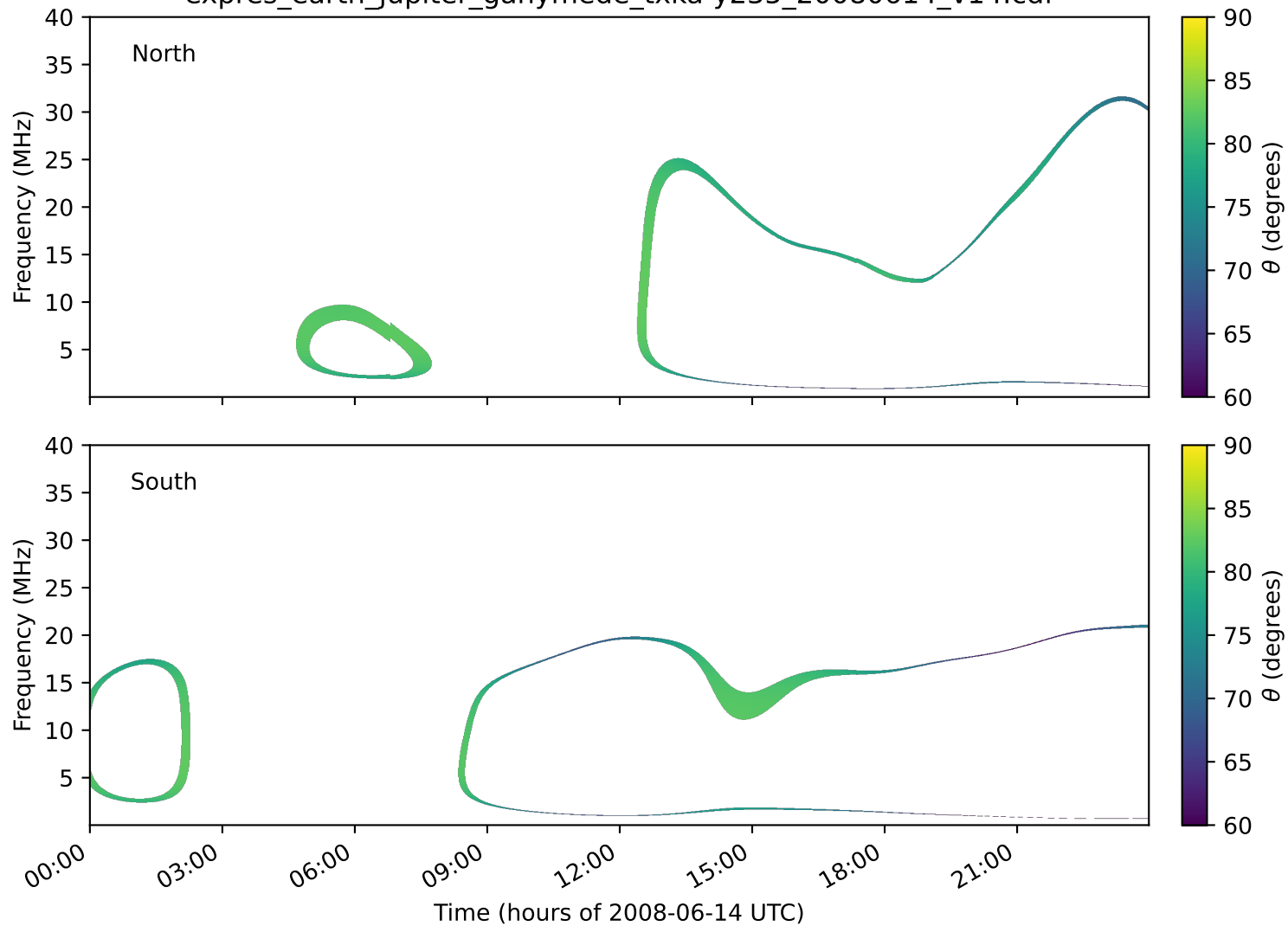
expres_earth_jupiter_ganymede_txka-y235_20080614_v14.cdf
