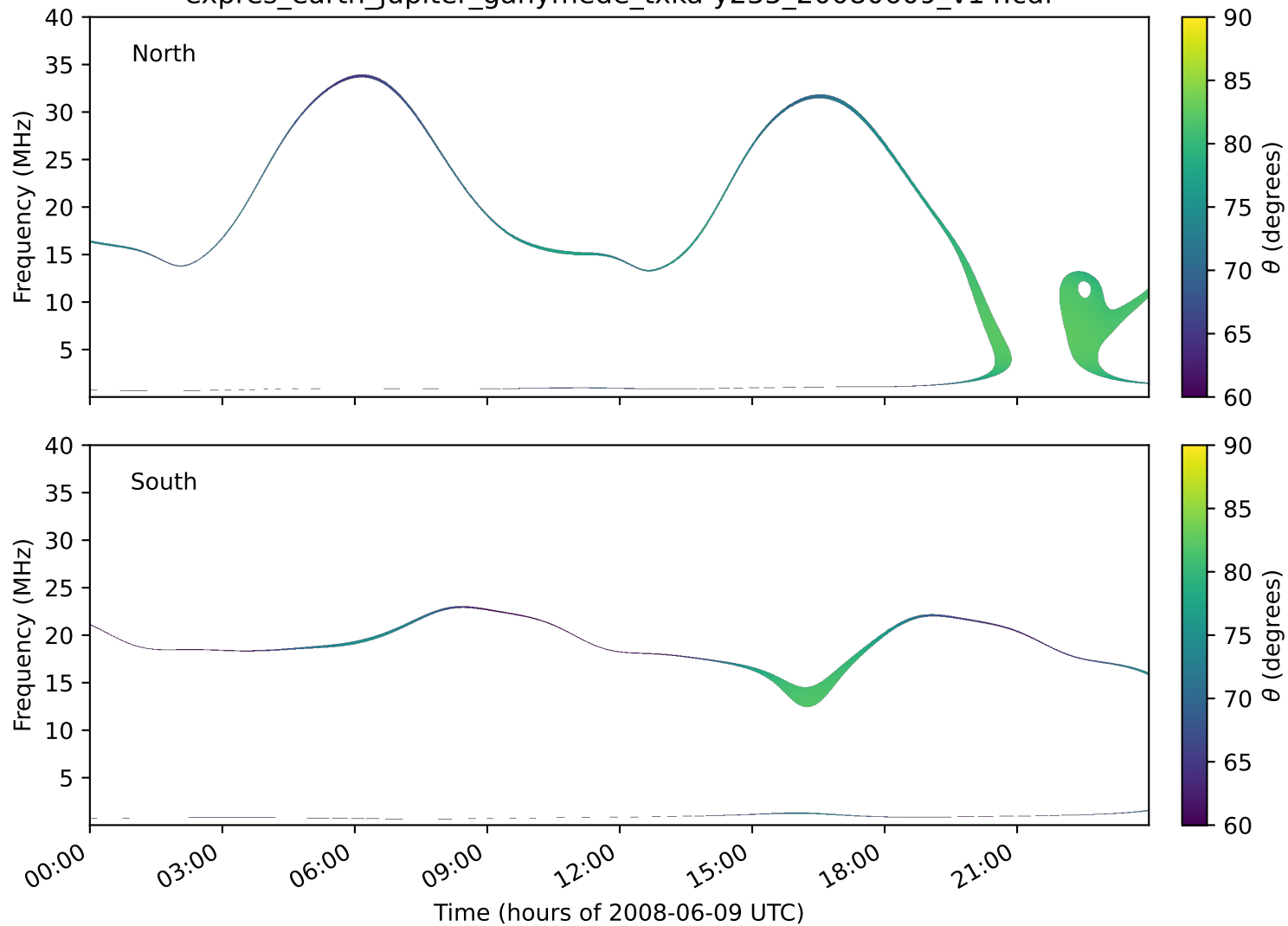
expres_earth_jupiter_ganymede_txka-y235_20080609_v14.cdf
