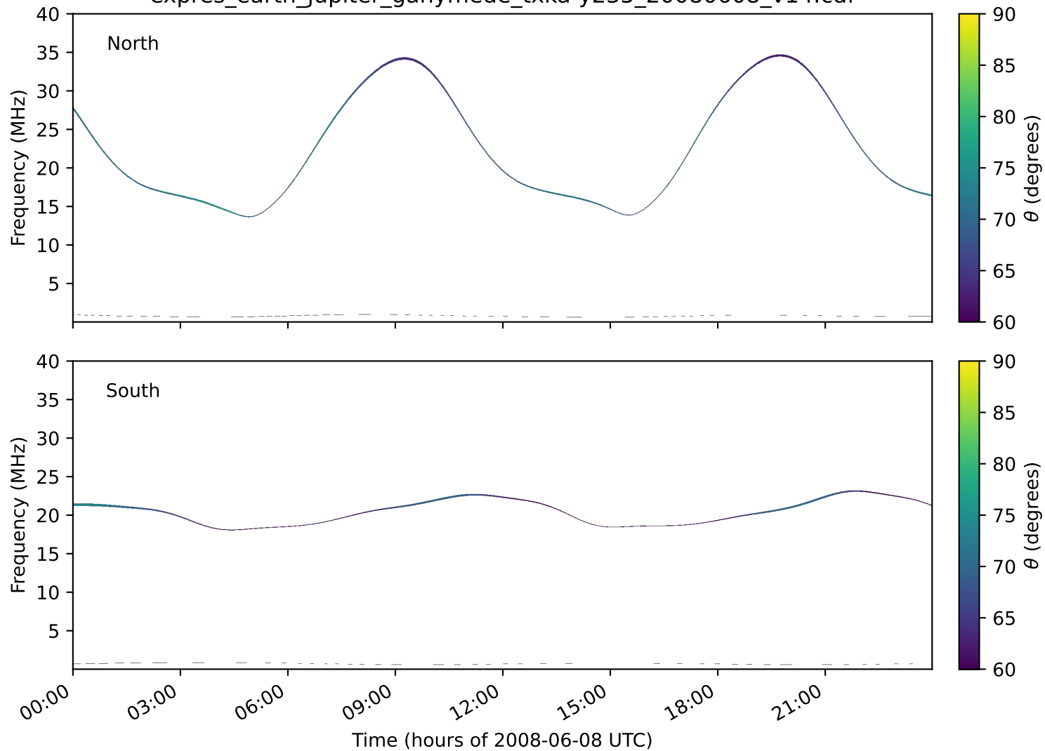
expres_earth_jupiter_ganymede_txka-y235_20080608_v14.cdf
