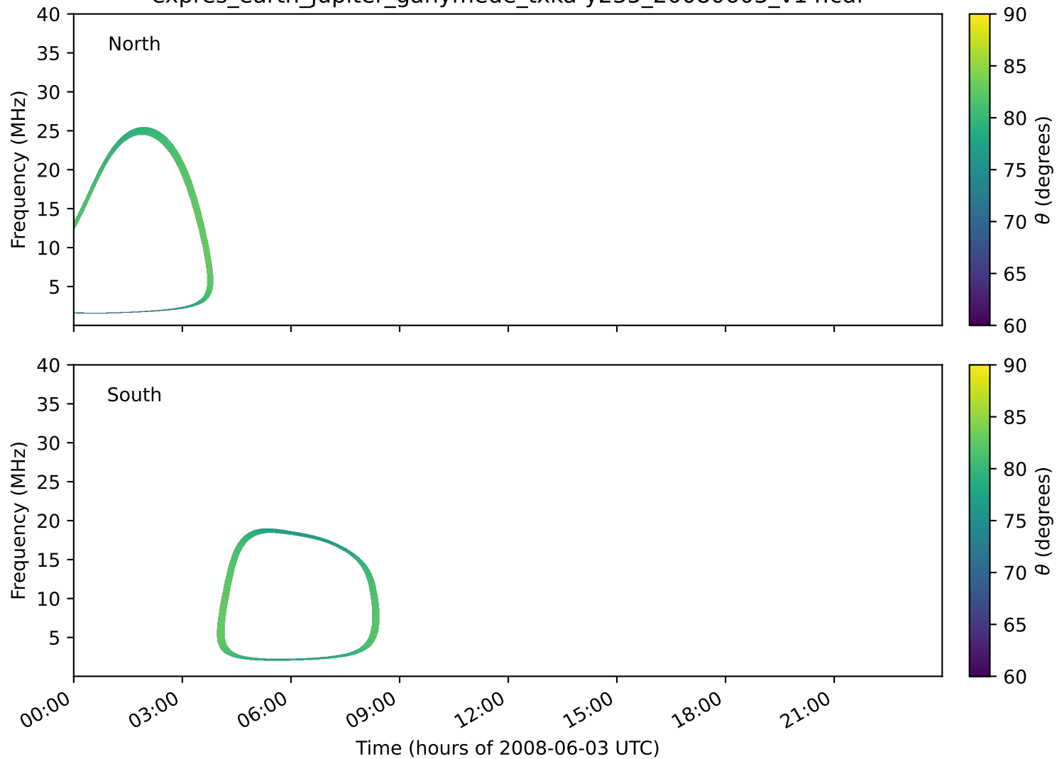
expres_earth_jupiter_ganymede_txka-y235_20080603_v14.cdf
