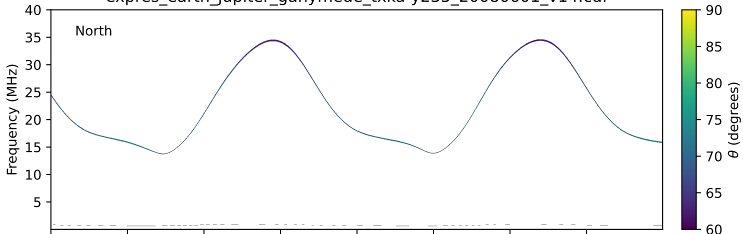
expres_earth_jupiter_ganymede_txka-y235_20080601_v14.cdf
