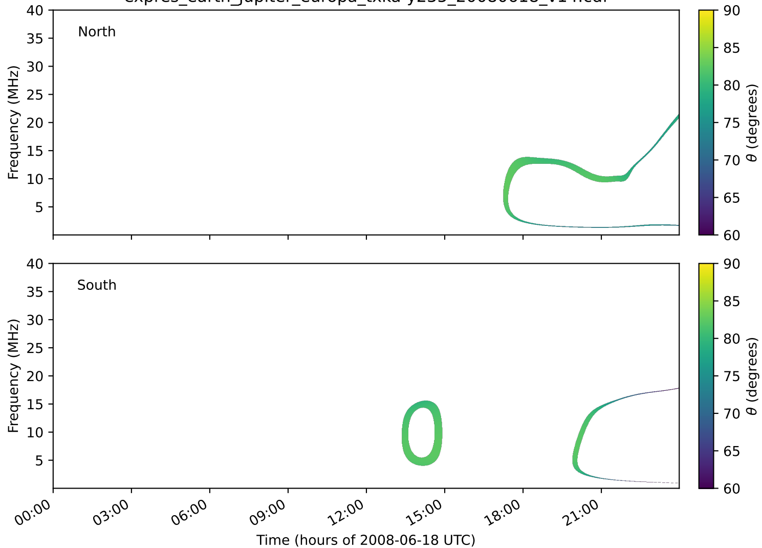
expres_earth_jupiter_europa_txka-y235_20080618_v14.cdf
