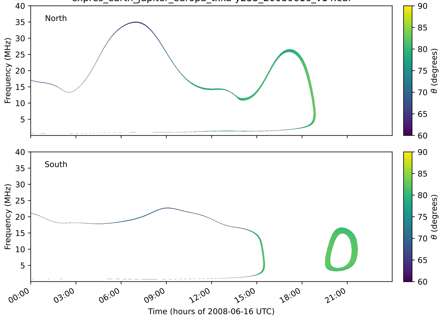
expres_earth_jupiter_europa_txka-y235_20080616_v14.cdf
