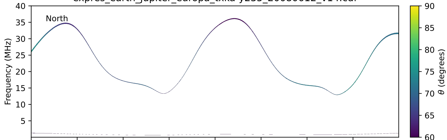
expres_earth_jupiter_europa_txka-y235_20080612_v14.cdf
