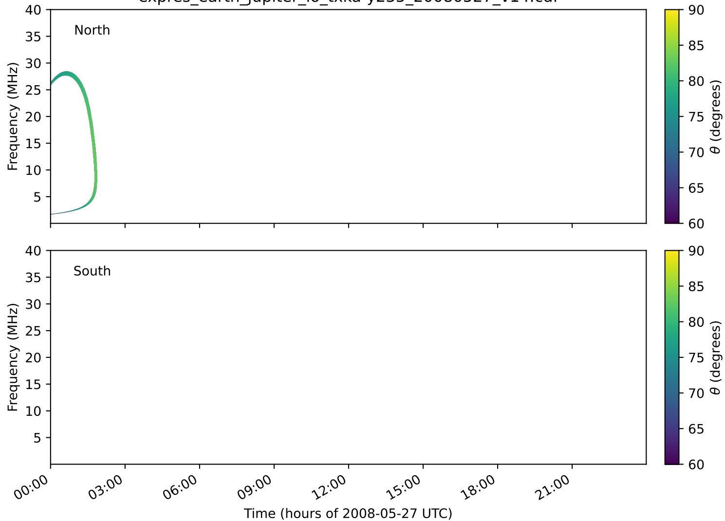
expres_earth_jupiter_io_txka-y235_20080527_v14.cdf
