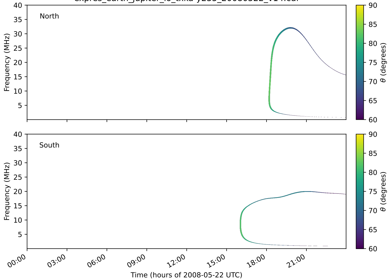
expres_earth_jupiter_io_txka-y235_20080522_v14.cdf
