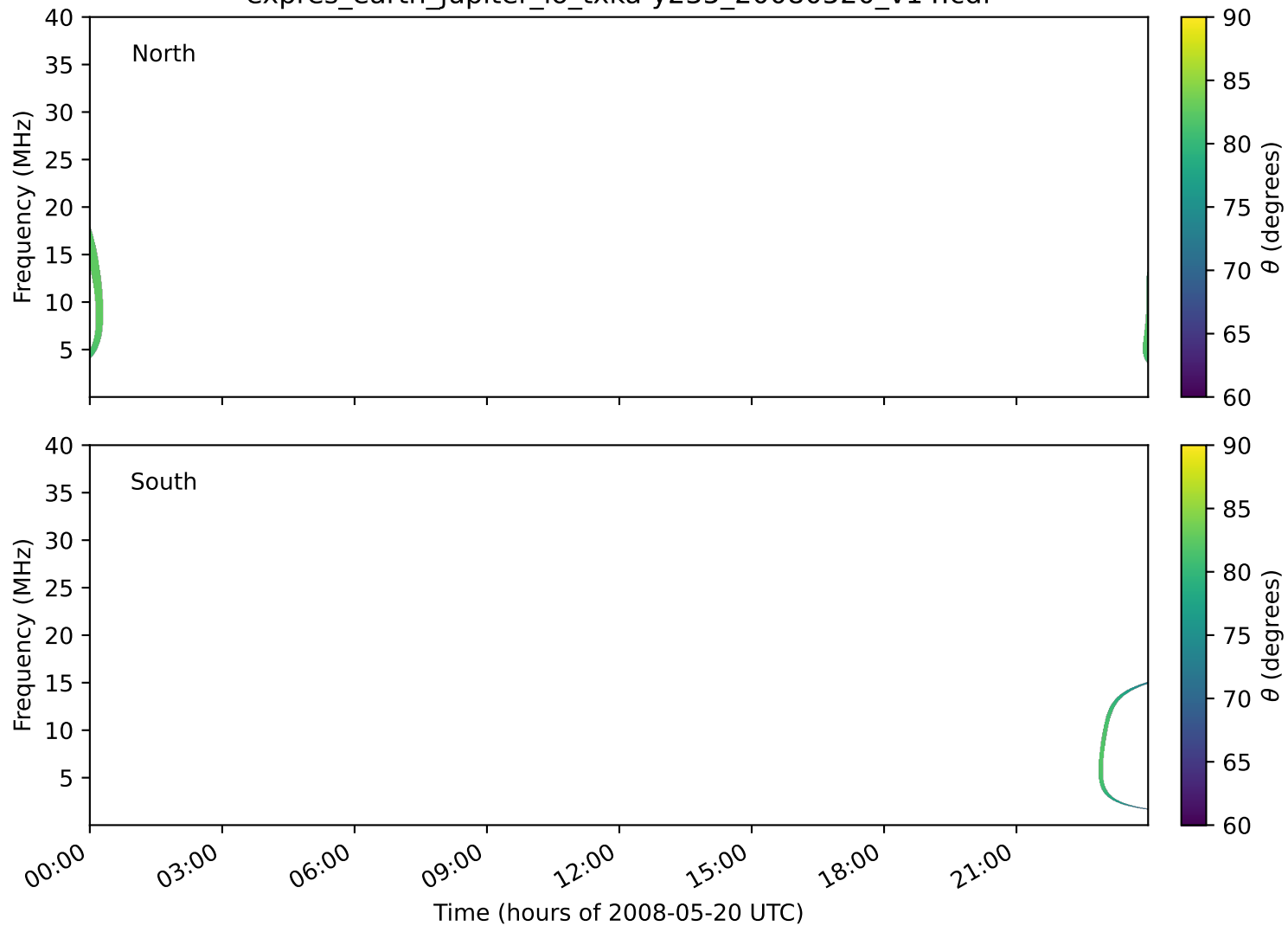
expres_earth_jupiter_io_txka-y235_20080520_v14.cdf
