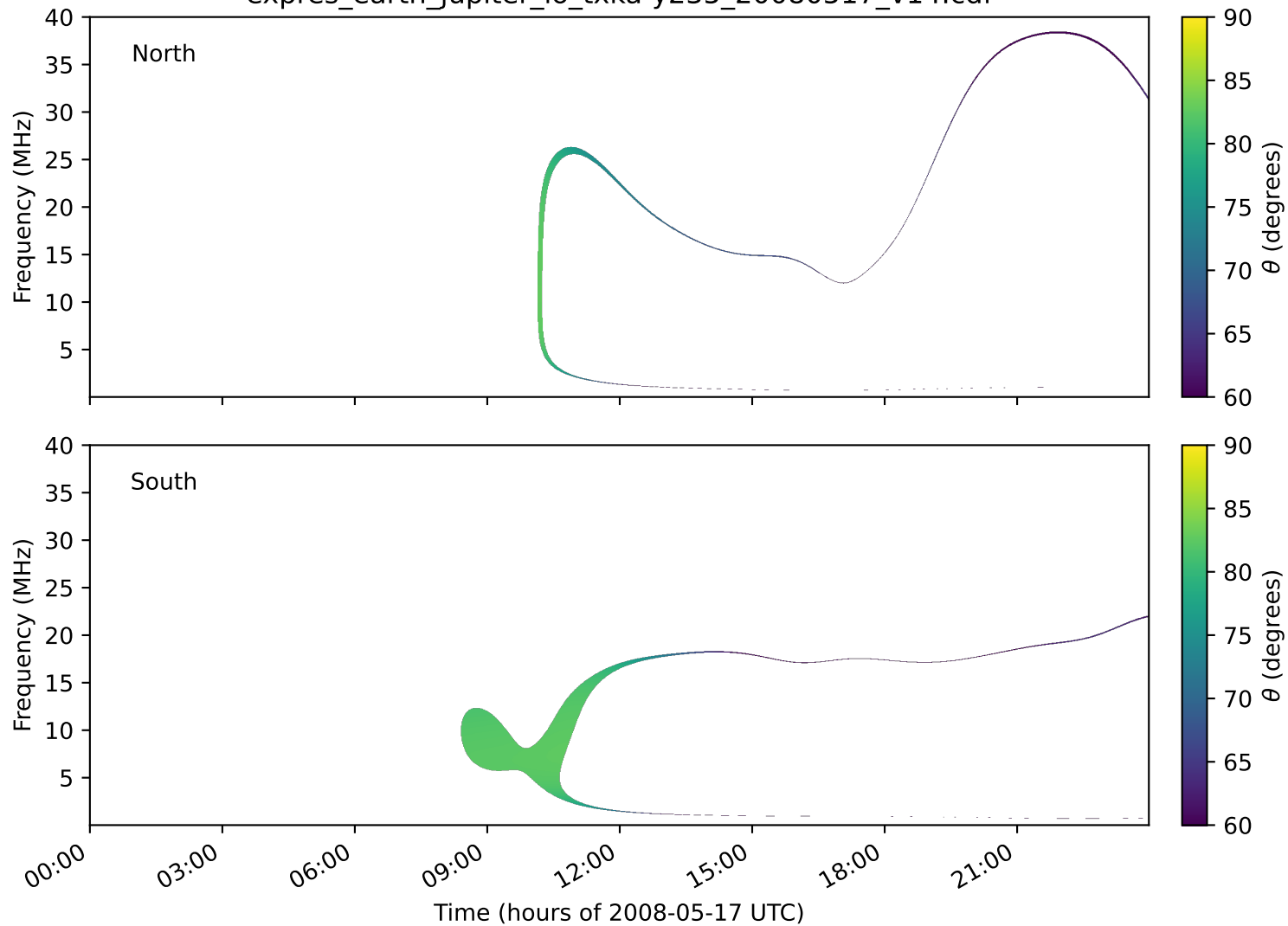
expres_earth_jupiter_io_txka-y235_20080517_v14.cdf
