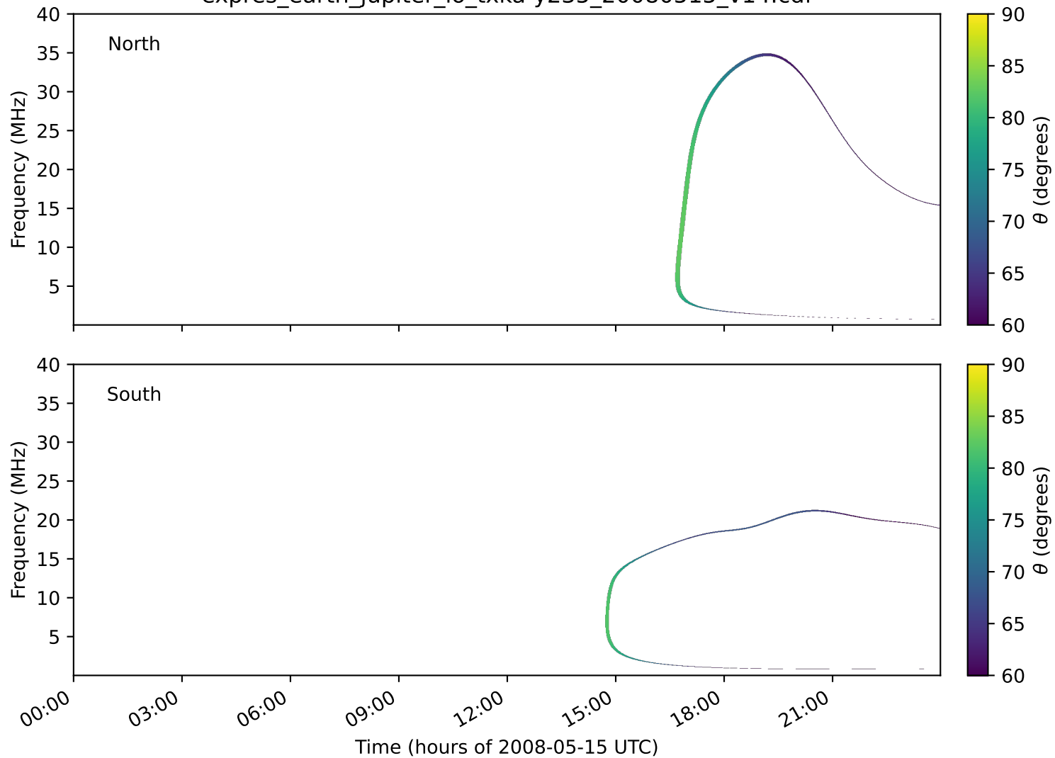
expres_earth_jupiter_io_txka-y235_20080515_v14.cdf
