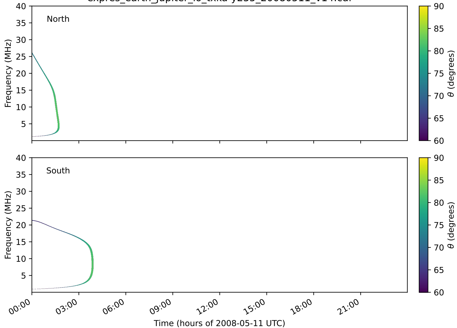
expres_earth_jupiter_io_txka-y235_20080511_v14.cdf
