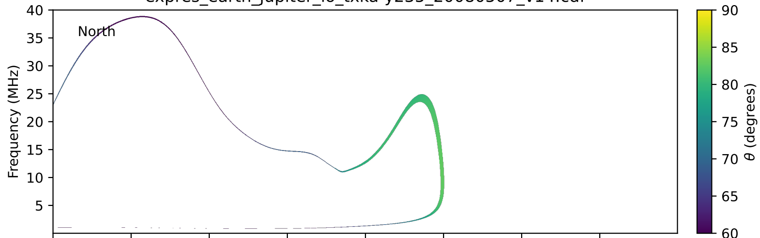
expres_earth_jupiter_io_txka-y235_20080507_v14.cdf
