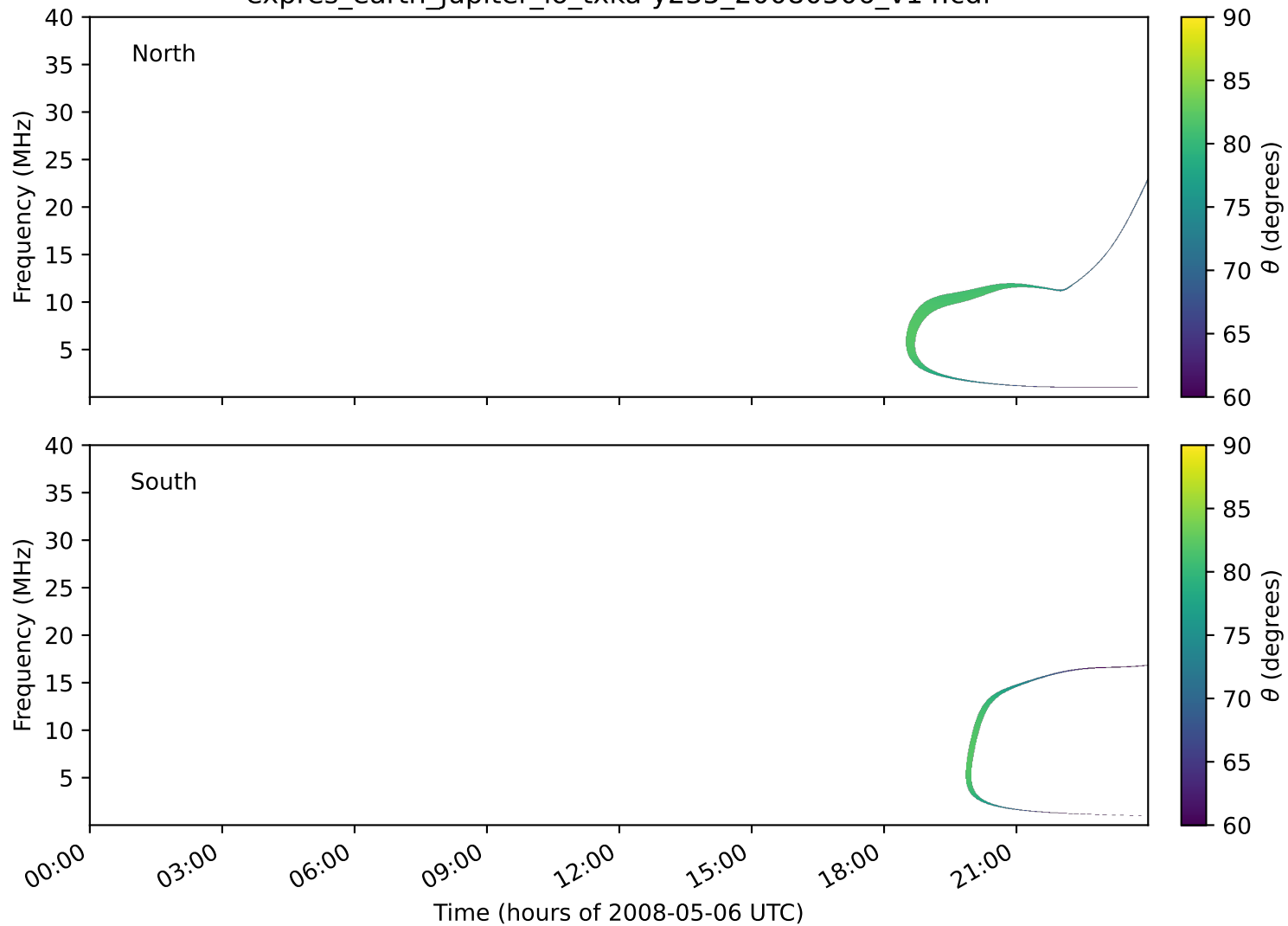
expres_earth_jupiter_io_txka-y235_20080506_v14.cdf
