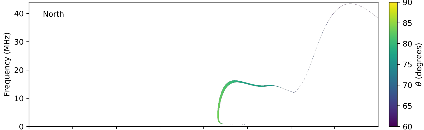
expres_earth_jupiter_io_jrm09_lossc-wid1deg_3kev_20080531_v01.cdf
