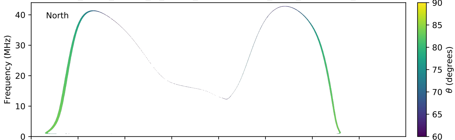
expres_earth_jupiter_io_jrm09_lossc-wid1deg_3kev_20080528_v01.cdf
