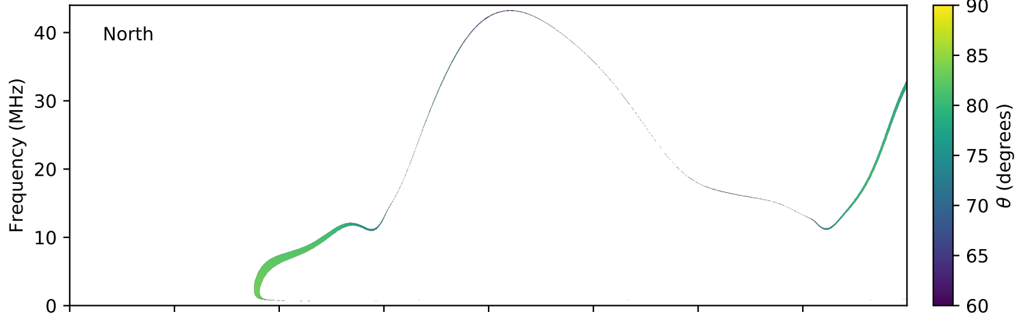
expres_earth_jupiter_io_jrm09_lossc-wid1deg_3kev_20080526_v01.cdf
