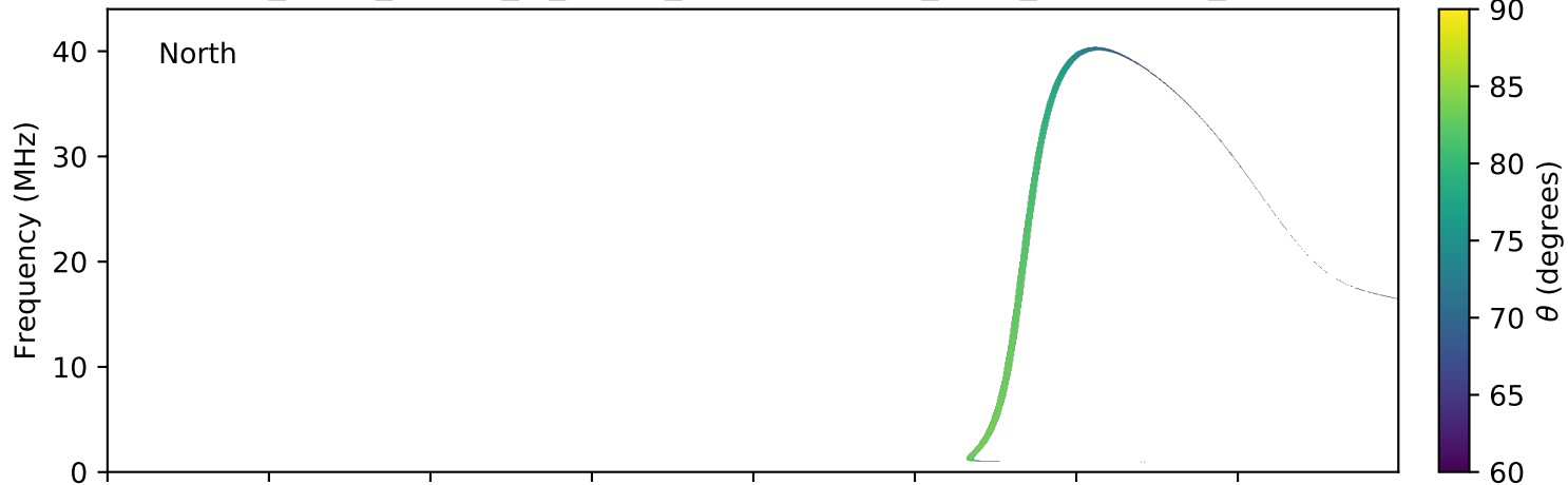
expres_earth_jupiter_io_jrm09_lossc-wid1deg_3kev_20080515_v01.cdf
