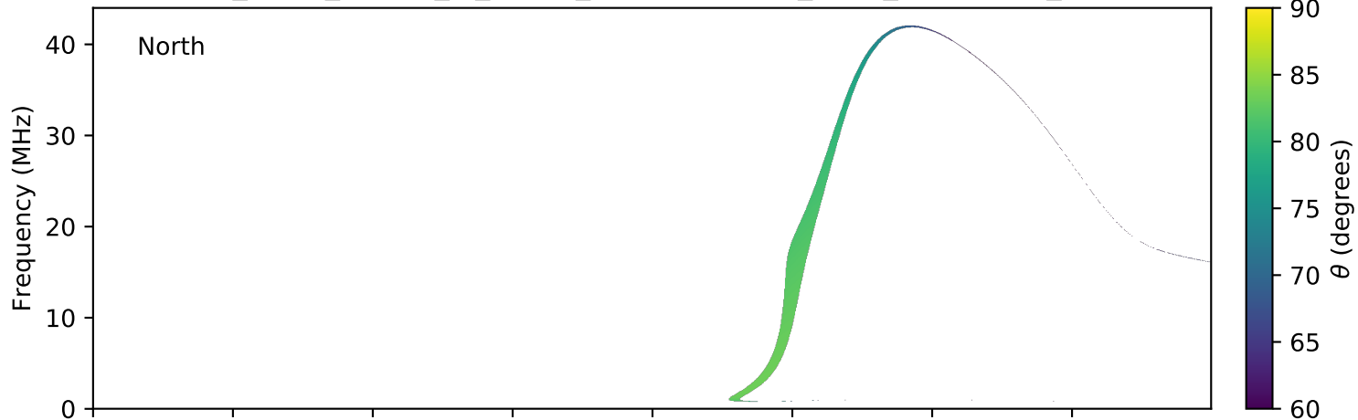
expres_earth_jupiter_io_jrm09_lossc-wid1deg_3kev_20080508_v01.cdf
