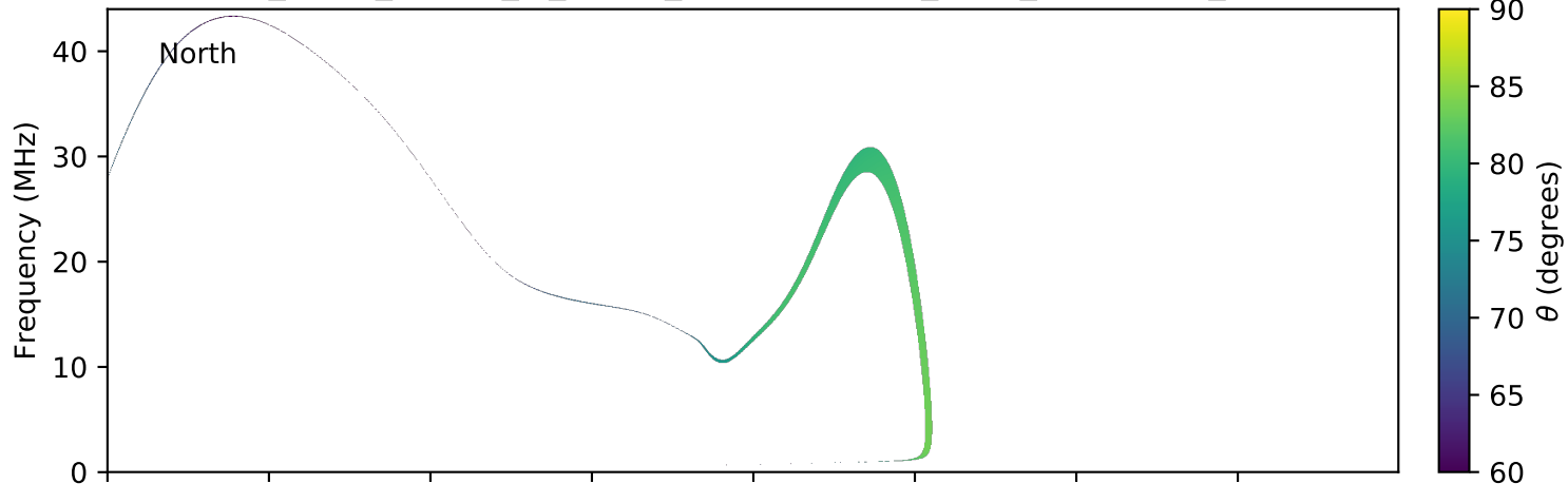
expres_earth_jupiter_io_jrm09_lossc-wid1deg_3kev_20080507_v01.cdf
