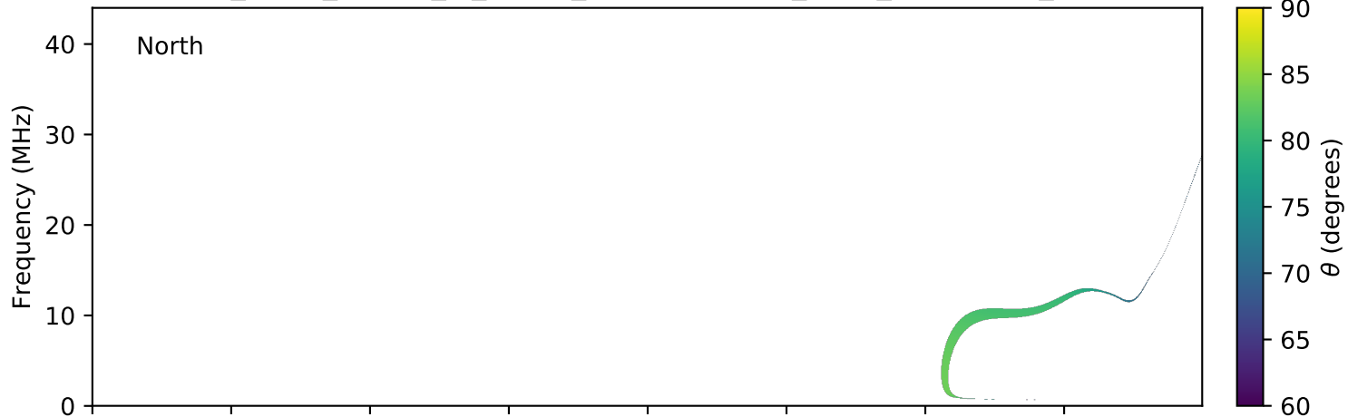
expres_earth_jupiter_io_jrm09_lossc-wid1deg_3kev_20080506_v01.cdf
