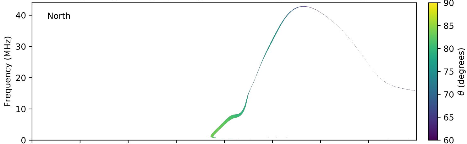
expres_earth_jupiter_io_jrm09_lossc-wid1deg_3kev_20080501_v01.cdf
