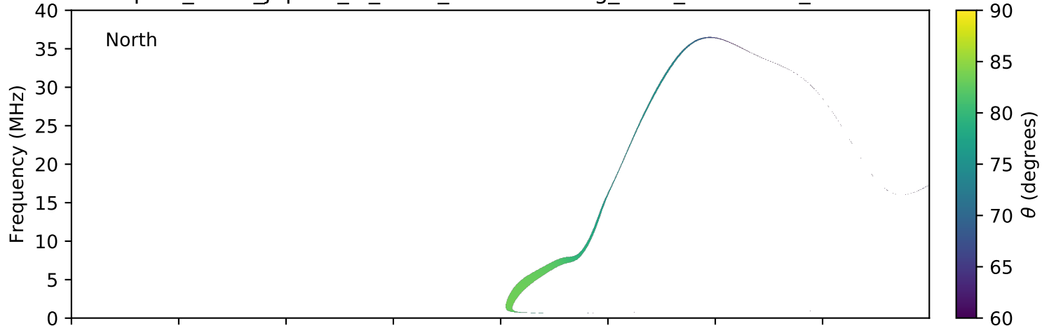
expres_earth_jupiter_io_isaac_lossc-wid1deg_3kev_20080531_v01.cdf
