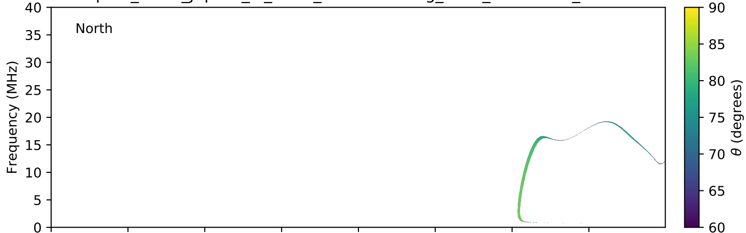
expres_earth_jupiter_io_isaac_lossc-wid1deg_3kev_20080529_v01.cdf
