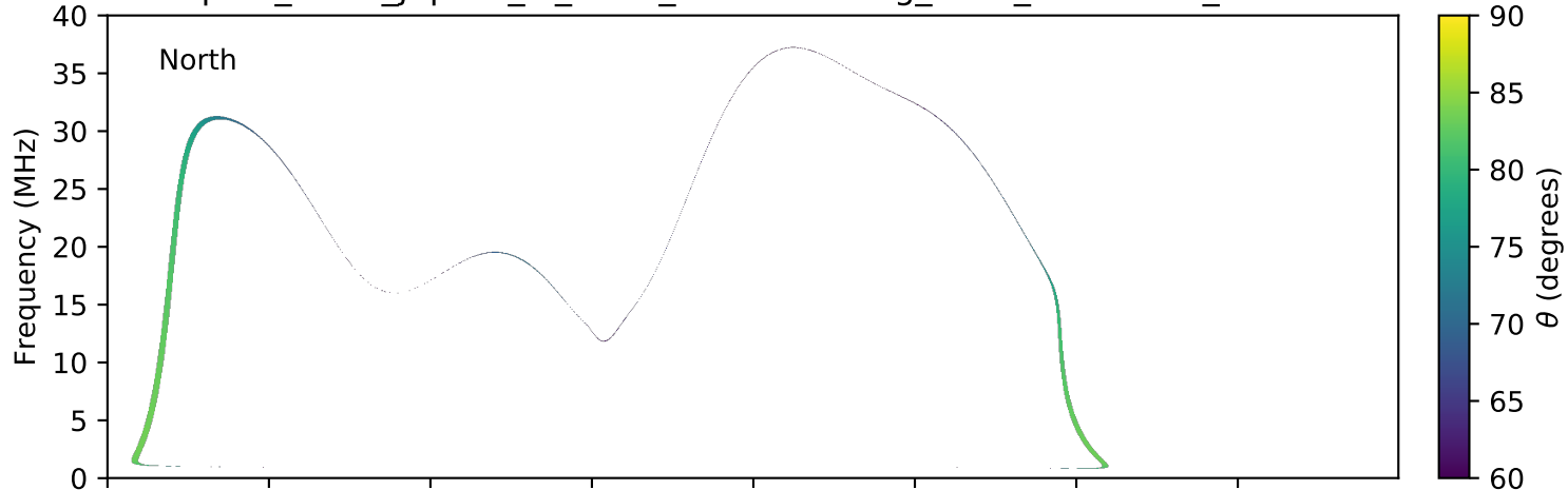
expres_earth_jupiter_io_isaac_lossc-wid1deg_3kev_20080528_v01.cdf
