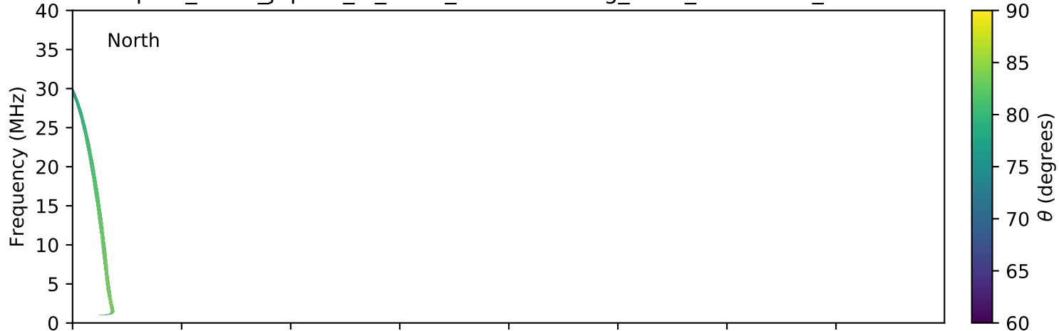
expres_earth_jupiter_io_isaac_lossc-wid1deg_3kev_20080527_v01.cdf
