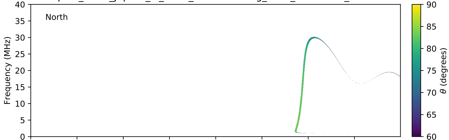
expres_earth_jupiter_io_isaac_lossc-wid1deg_3kev_20080522_v01.cdf
