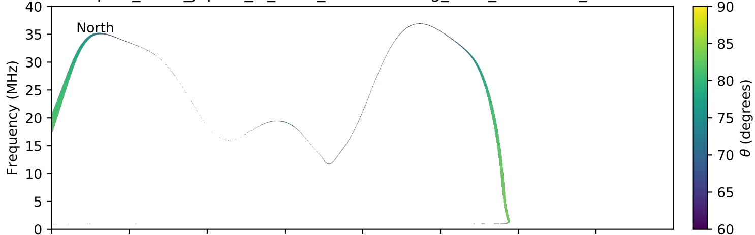
expres_earth_jupiter_io_isaac_lossc-wid1deg_3kev_20080521_v01.cdf
