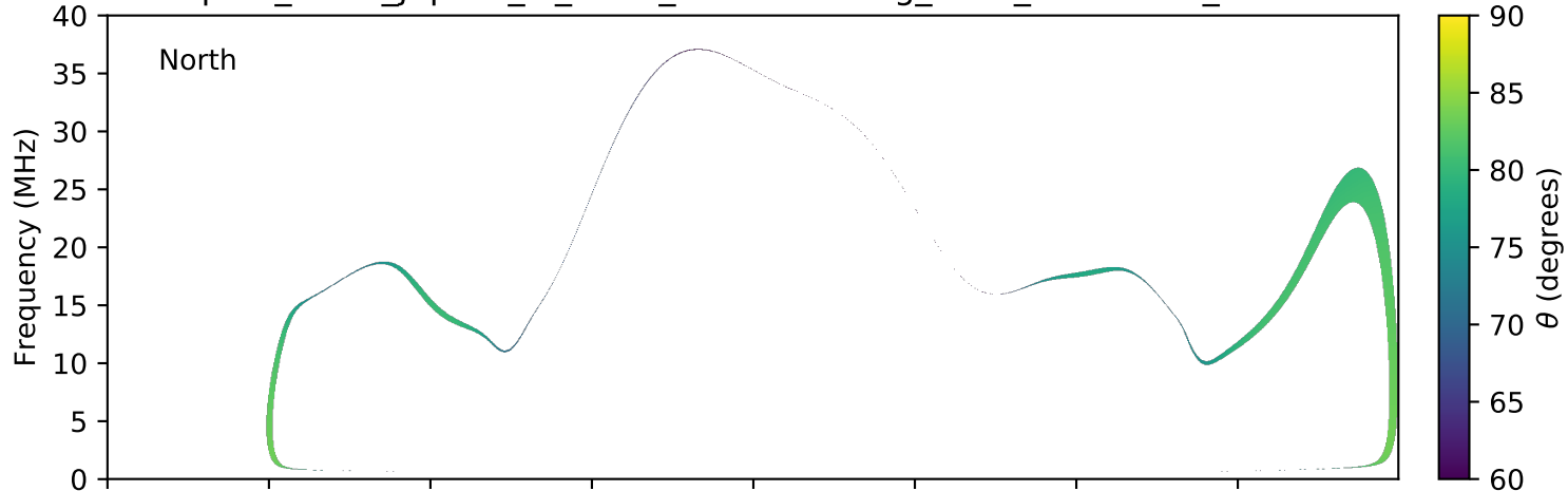
expres_earth_jupiter_io_isaac_lossc-wid1deg_3kev_20080519_v01.cdf
