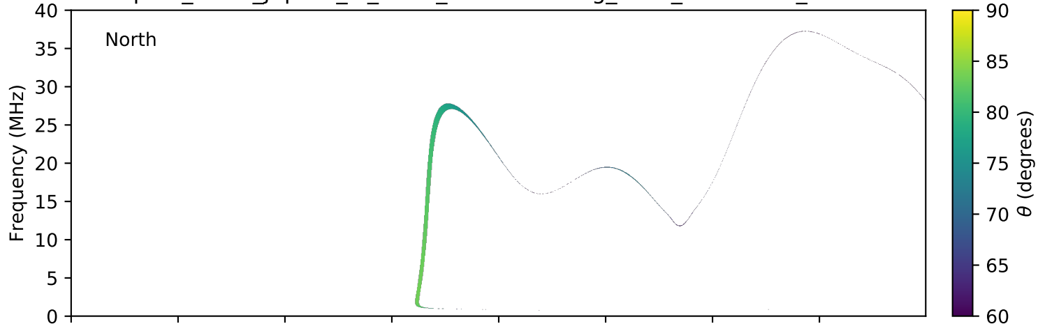
expres_earth_jupiter_io_isaac_lossc-wid1deg_3kev_20080517_v01.cdf
