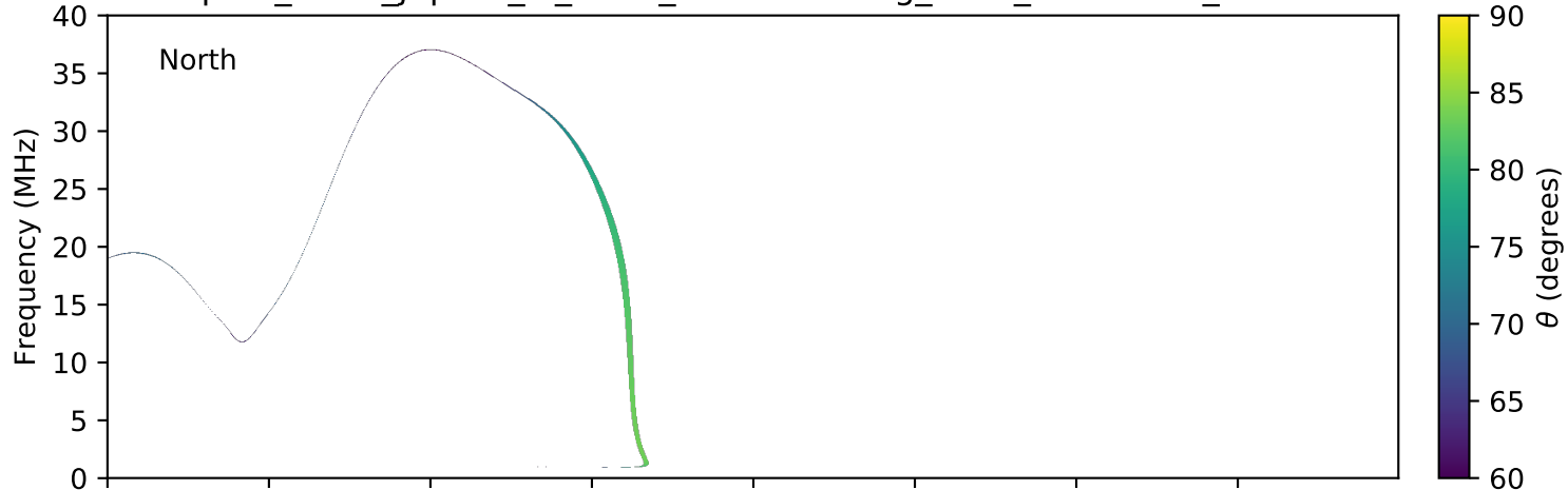
expres_earth_jupiter_io_isaac_lossc-wid1deg_3kev_20080516_v01.cdf
