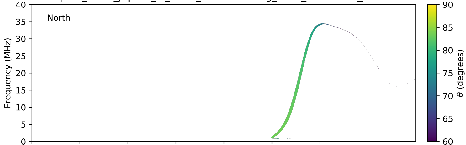
expres_earth_jupiter_io_isaac_lossc-wid1deg_3kev_20080515_v01.cdf
