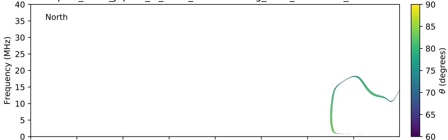
expres_earth_jupiter_io_isaac_lossc-wid1deg_3kev_20080513_v01.cdf
