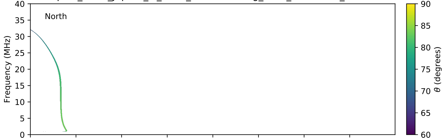
expres_earth_jupiter_io_isaac_lossc-wid1deg_3kev_20080511_v01.cdf
