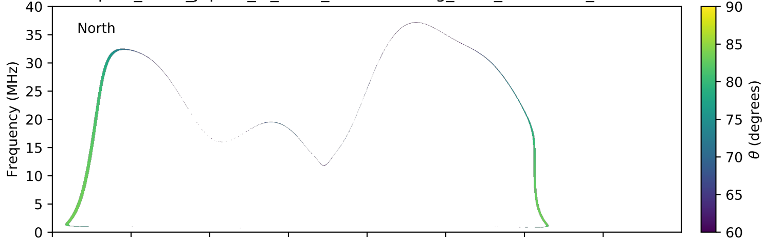
expres_earth_jupiter_io_isaac_lossc-wid1deg_3kev_20080505_v01.cdf
