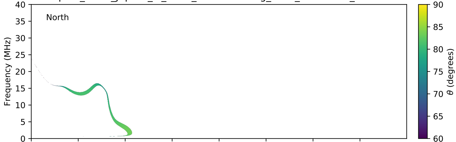
expres_earth_jupiter_io_isaac_lossc-wid1deg_3kev_20080502_v01.cdf
