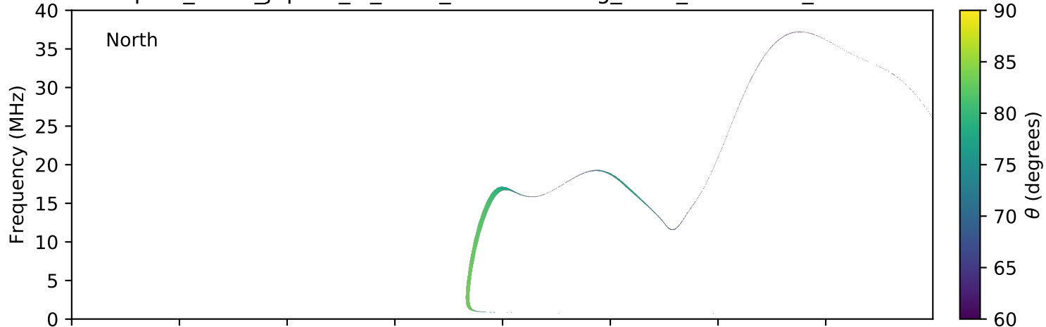
expres_earth_jupiter_io_isaac_lossc-wid1deg_3kev_20080501_v01.cdf
