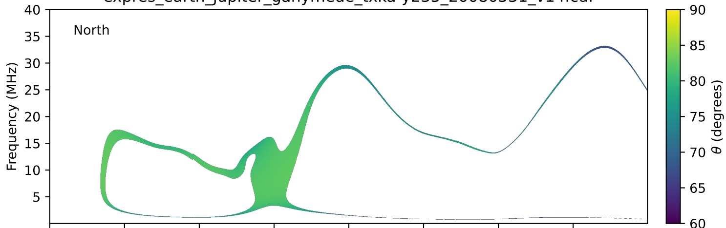
expres_earth_jupiter_ganymede_txka-y235_20080531_v14.cdf
