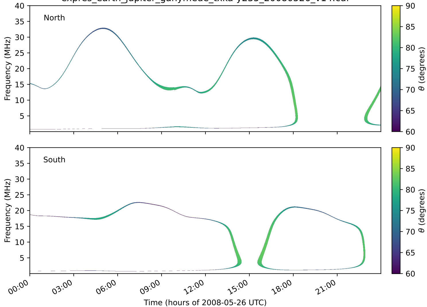
expres_earth_jupiter_ganymede_txka-y235_20080526_v14.cdf
