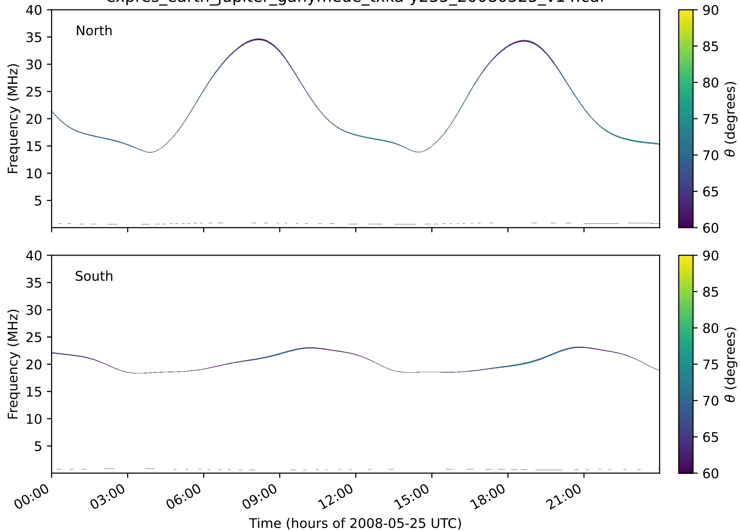
expres_earth_jupiter_ganymede_txka-y235_20080525_v14.cdf
