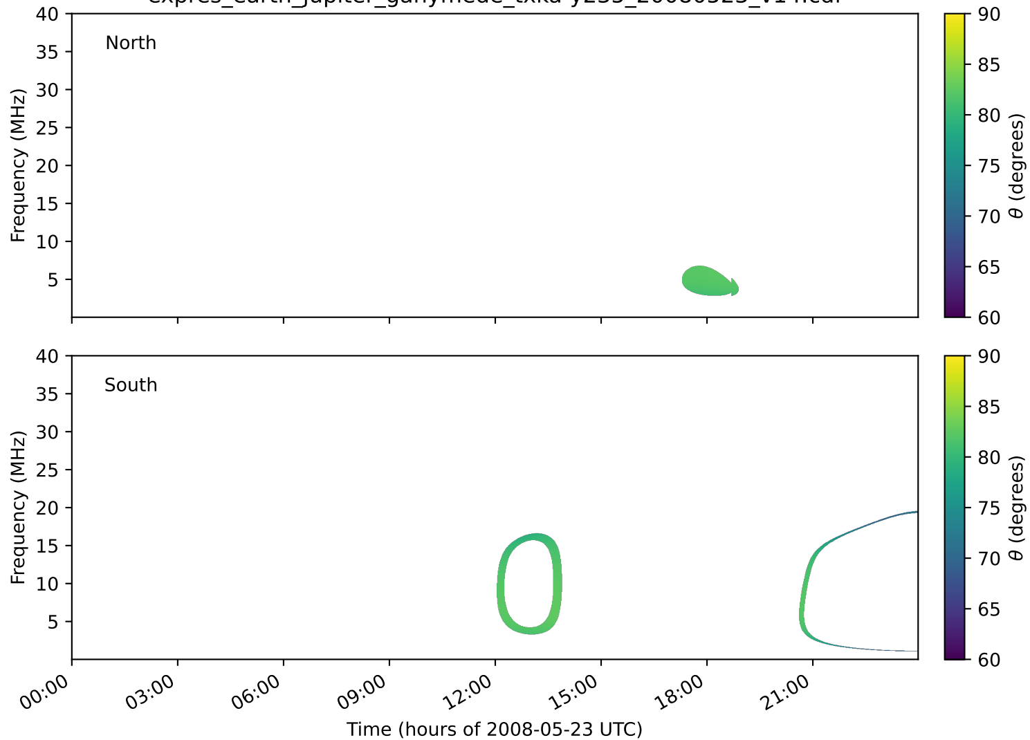
expres_earth_jupiter_ganymede_txka-y235_20080523_v14.cdf
