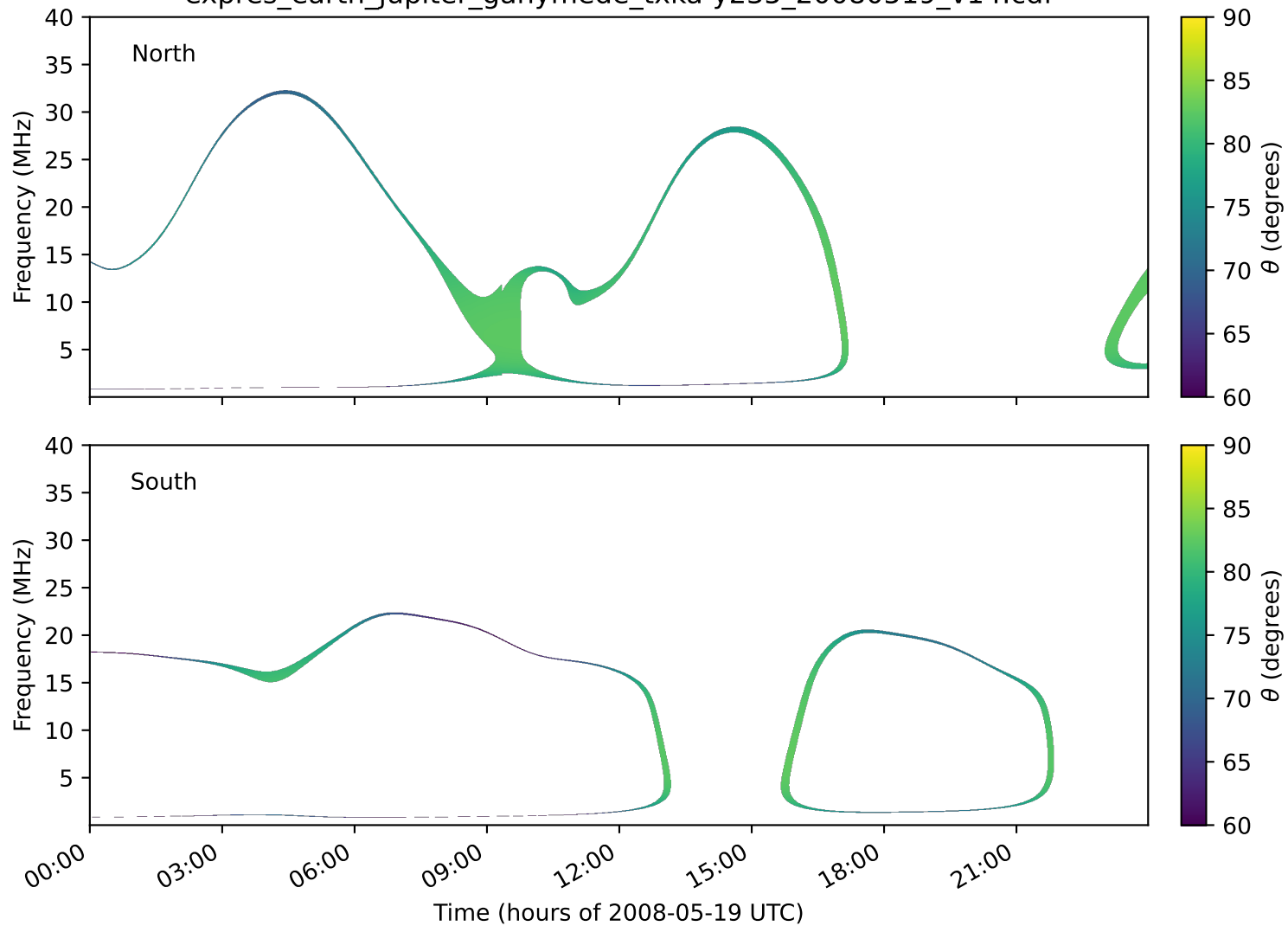
expres_earth_jupiter_ganymede_txka-y235_20080519_v14.cdf
