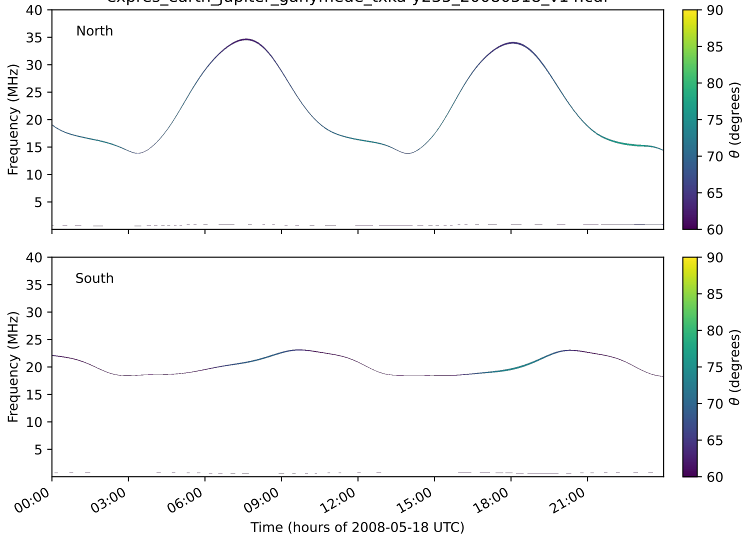
expres_earth_jupiter_ganymede_txka-y235_20080518_v14.cdf
