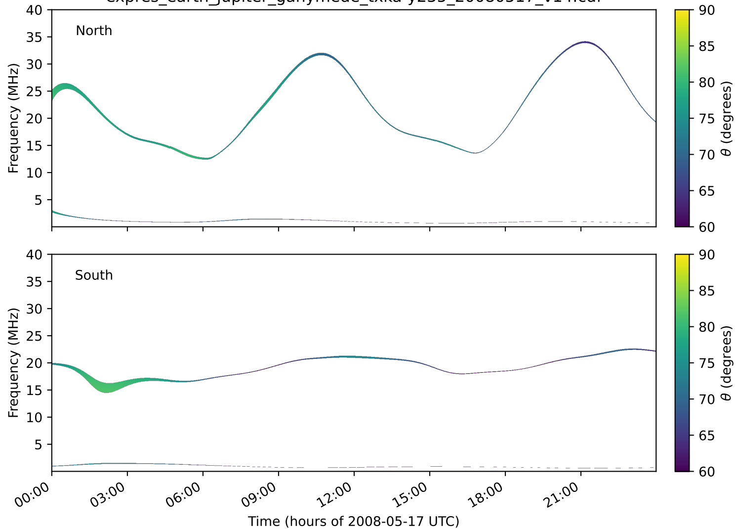
expres_earth_jupiter_ganymede_txka-y235_20080517_v14.cdf
