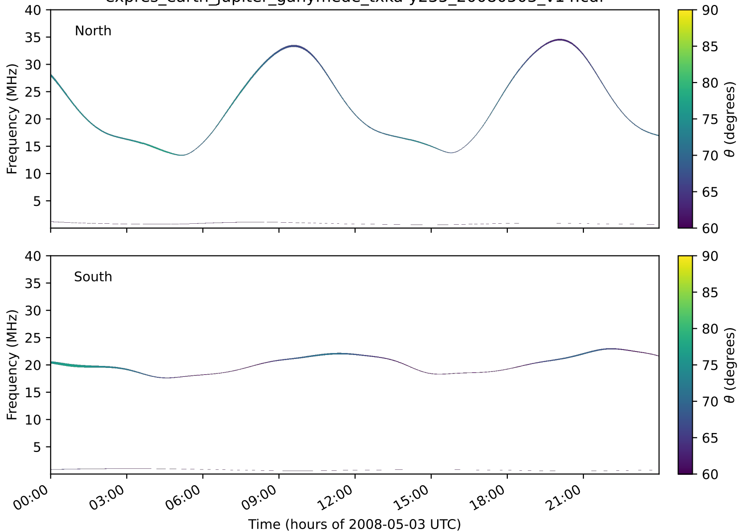
expres_earth_jupiter_ganymede_txka-y235_20080503_v14.cdf
