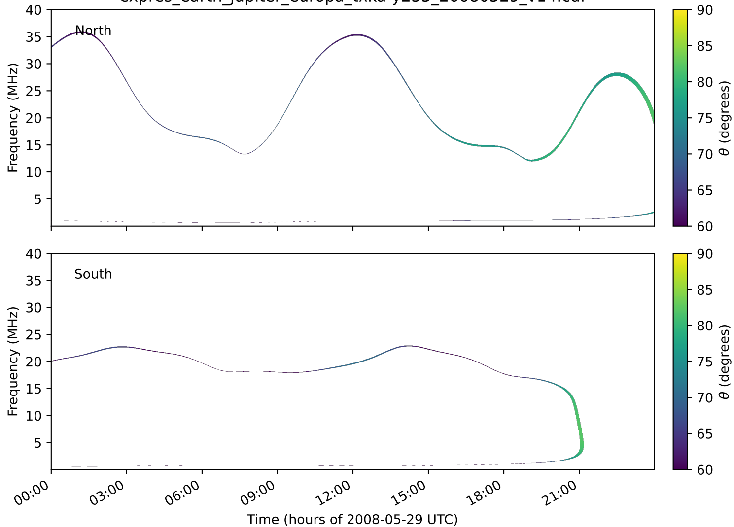
expres_earth_jupiter_europa_txka-y235_20080529_v14.cdf
