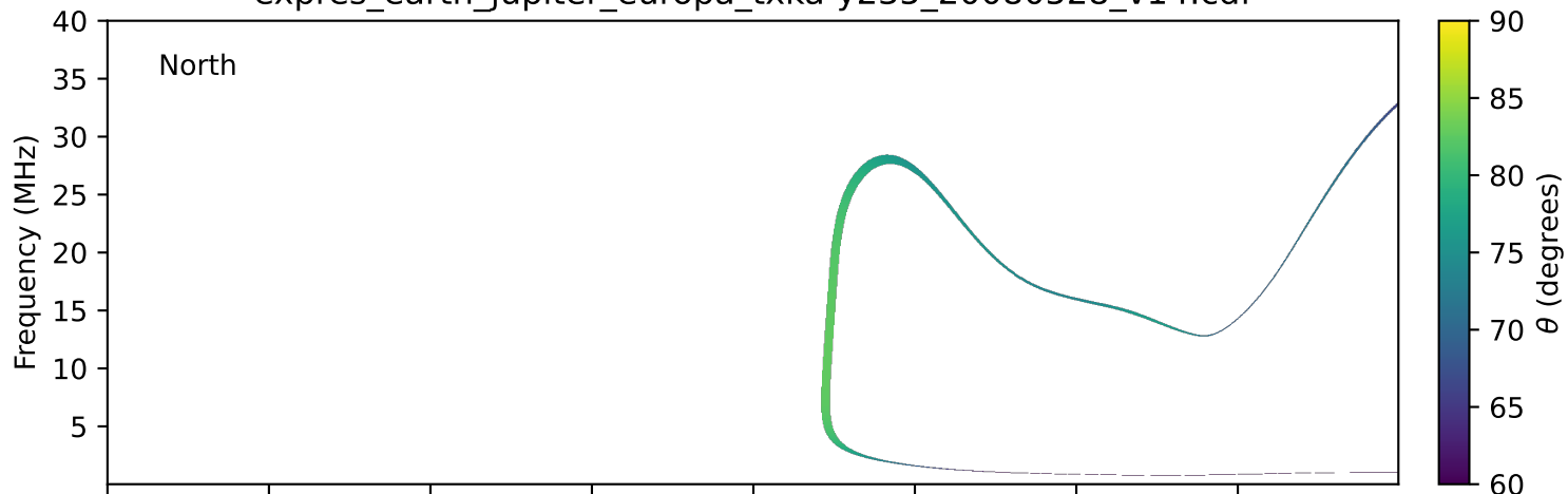
expres_earth_jupiter_europa_txka-y235_20080528_v14.cdf
