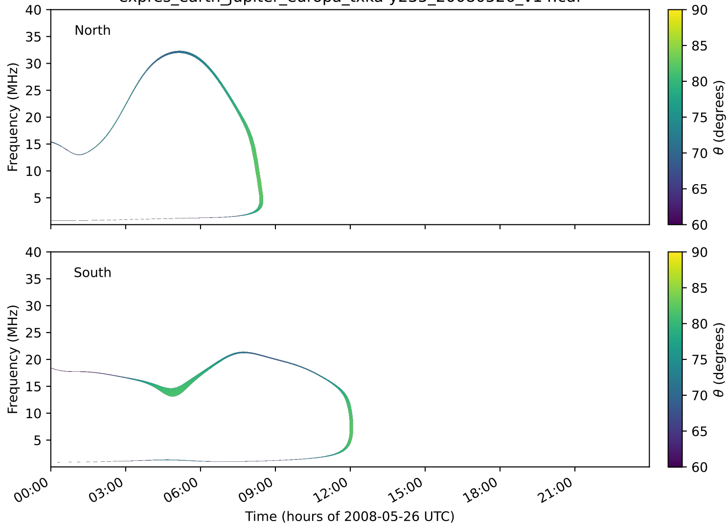
expres_earth_jupiter_europa_txka-y235_20080526_v14.cdf
